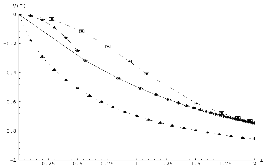
Figure 8.2: The dependence of the selection variance V on the selection intensity I for tournament selection ( \diamond — \diamond ), truncation selection ( \triangle - - \triangle ), ranking selection ( \star - - \star ), and exponential ranking selection ( \square - - \square ). Note that for tournament selection only the dotted points on the graph correspond to valid (integer) tournament sizes.
